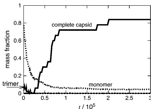
FIGURE 13 The mass fraction of monomers, trimers, and complete capsids (60 subunits, with n_b = 4 bonds each) as a function of time, t , for design B_4 , illustrating that intermediate concentrations are always small during successful assembly. The parameters are those given in Fig. 9.
