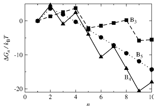
FIGURE 12 Free energy projections onto the number of particles in a capsid, n , for each design, relative to monomers in solution at C_0 = 0.11 with \theta_m = 0.5 . The values of \epsilon_b are the optimal values from Fig. 9: 16.0, 12.7, and 10.5 for the B_3 , B_4 , and B_5 designs, respectively. Free energies were obtained with Boltzmann weighted sums over configurations with a given cluster size as described in Appendix C. Lines are drawn between the points as a guide to the eye.
