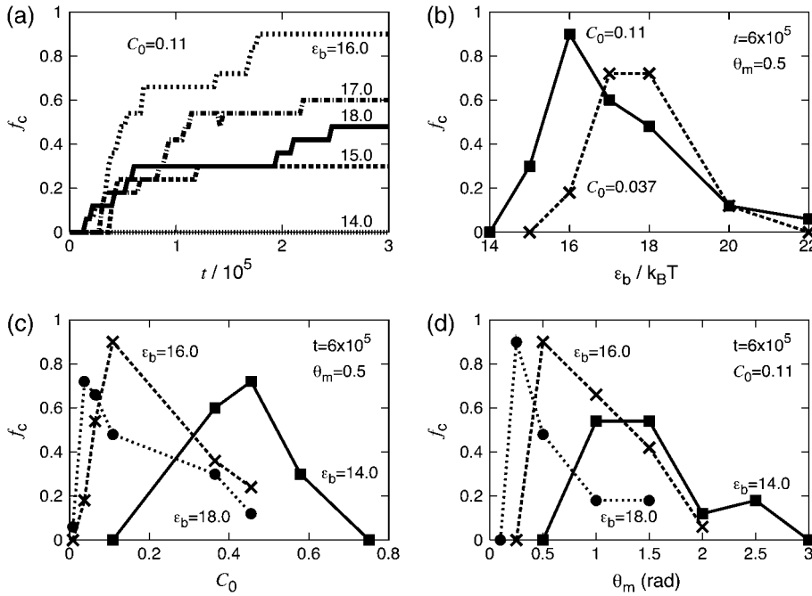
FIGURE 6 Examples of the influence of system parameters on assembly dynamics for design B3. (a) The fraction of complete capsids versus time, f_c , is shown for \theta_m = 0.5 and C_0 = N\sigma^3/L^3 = 0.11 at varying \epsilon_b illustrating the sigmoidal shape of capsid yields. Note that variations of f_c are in discrete units of 0.06 because there are 1000 subunits and each complete capsid has 60 subunits. Variation of the final mass fraction of complete capsids, f_c , is shown in panels b–d: (b) variation with C_0 = 0.11 and \theta_m = 0.5 , (c) variation with C_0 at several values of \epsilon_b with \theta_m = 0.5 , and (d) variation with \theta_m for several values of \epsilon_b and C_0 = 0.11 . Note that \epsilon_b does not denote the free energy to bind; there is a significant entropy penalty, calculated in Eq. 15.
