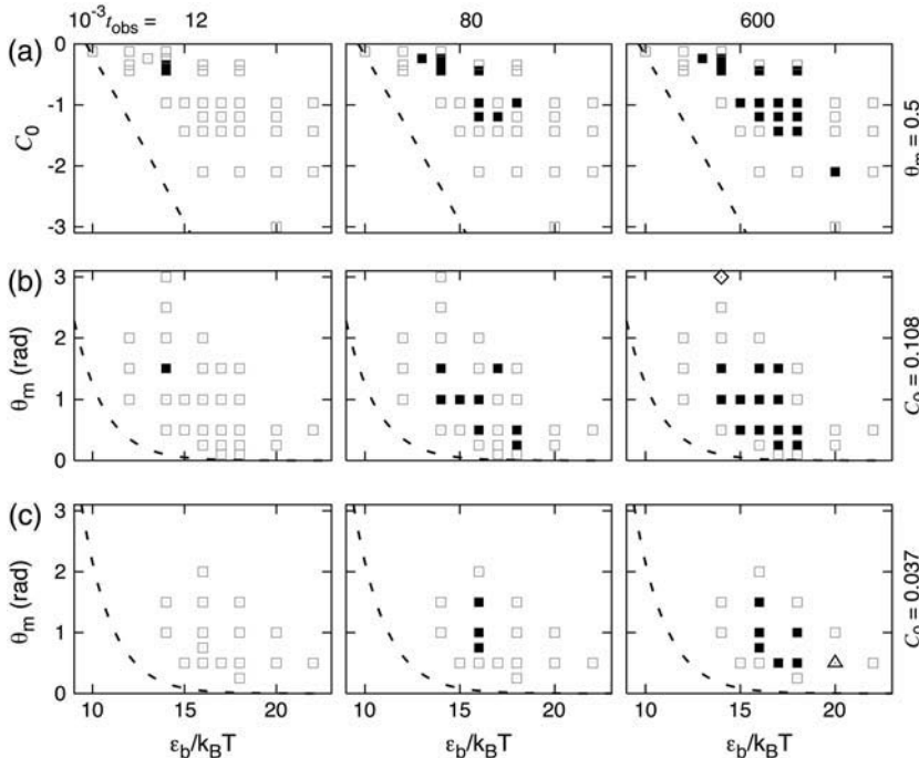
FIGURE 7 Changing model parameters reveals the kinetic phase diagram for design B3. Solid points denote parameter values for which 30% of subunits are in complete capsids ( f_c \geq 30\% ) by the observation time, t_{\text{obs}} , open points indicate parameter values for which f_c < 30\% , and the dashed lines indicate the location of the thermodynamic critical surface, calculated with Eq. 16. The first, second, and third columns correspond to observation time t_{\text{obs}} = 1.2 \times 10^4 , 8 \times 10^4 , and 6 \times 10^5 , respectively. The top row (a) shows cross sections through C_0 and \epsilon_b with \theta_m = 0.5 . The second and third row show cross sections through \theta_m and \epsilon_b , with (b) C_0 = 0.11 and (c) C_0 = 0.037 . In each case the region covered by solid points roughly defines a cross section of parameter space within which assembly is kinetically possible. Simulation snapshots corresponding to the \diamond in the right hand panel in row b and the \triangle in the right-hand panel in row a are shown in Fig. 8.
