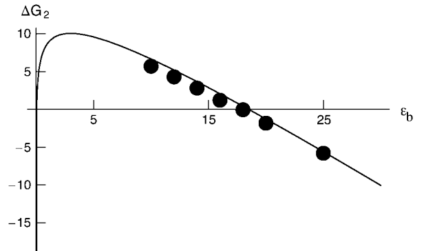
FIGURE 4 Binding free energies for dimerization calculated from Eqs. 14 and 15 (line) and Monte Carlo simulations (points). Free energies are with reference to a standard state with volume fraction of 1 and free rotational motion, and the maximum angle parameters, defined in Eq. 6, are \theta_m = \phi_m = 0.5 .
